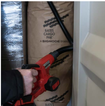
Portable battery inflator
